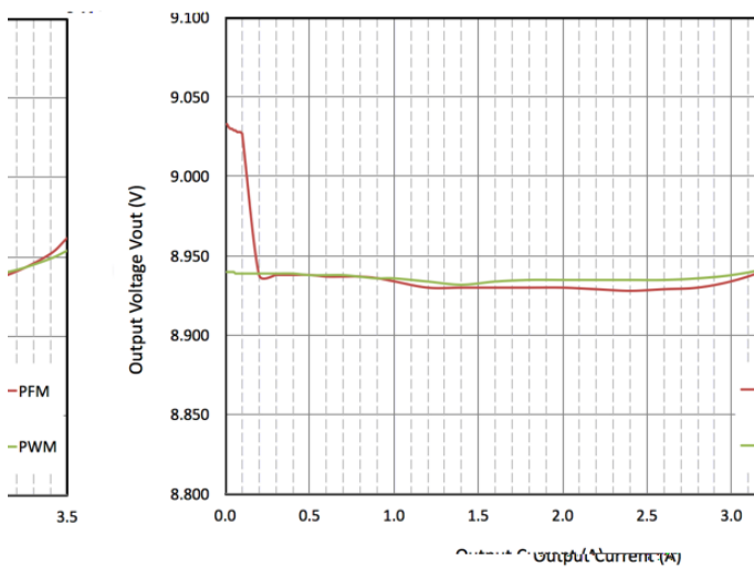
Figure 11. Load Regulation (Vin=3.6V, Vout=9V)
